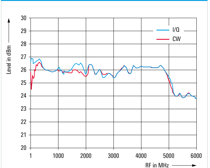
Measured maximum output power versus frequency
